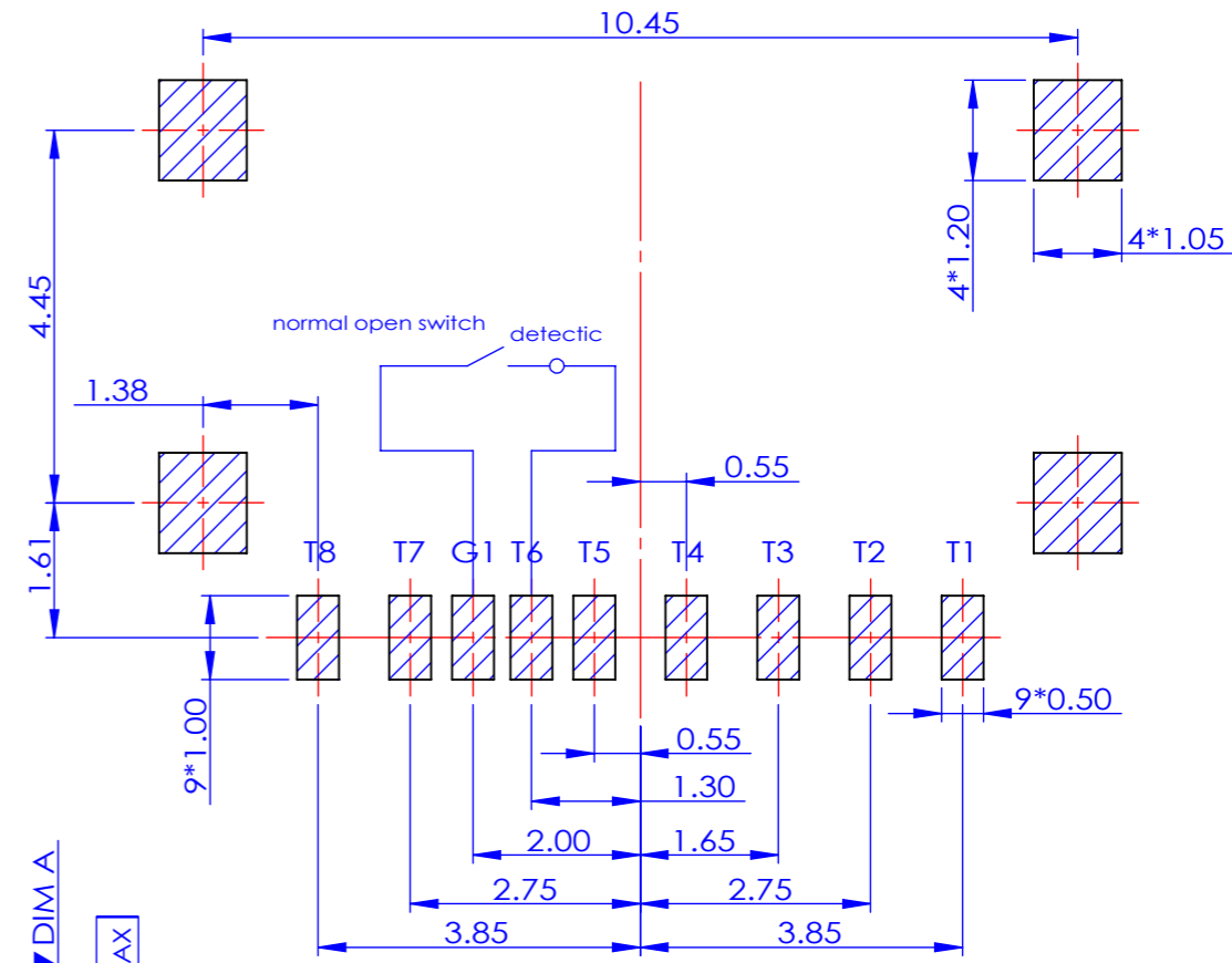
P.C.B LAYOUT ( TOLERANCE:±0.05 )
